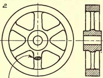
REVOLVED SECTION.
